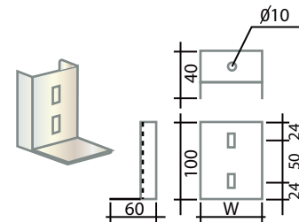
SPLICE PLATE SET
