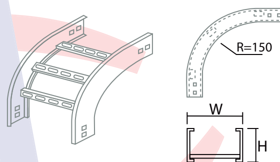
OUTSIDE RISER
