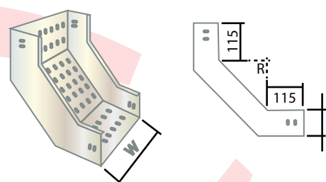
DIAGONAL
