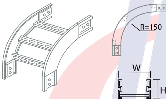
OUTSIDE RISER
