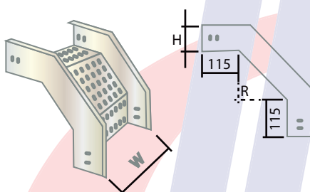
DIAGONAL
