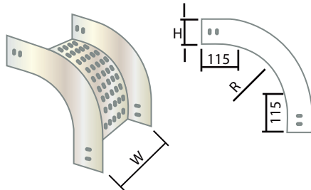
RADIUS
