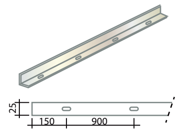
STRAIGHT SEPARATOR
