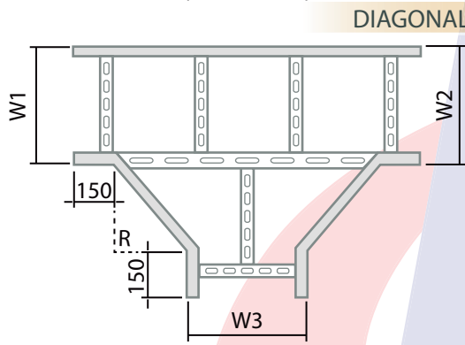
Radius Type
