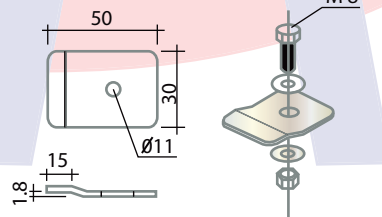
HOLD DOWN CLIP
