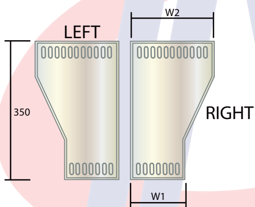
Offset Reducer
