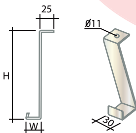
HOLD DOWN CLAMP
