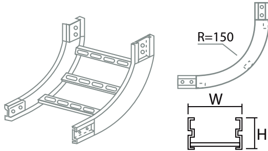
OUTSIDE RISER
