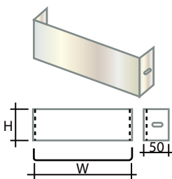
END PLATE SET
