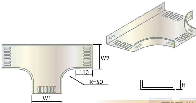
TEE TRAY
