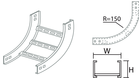
INSIDE RISER
