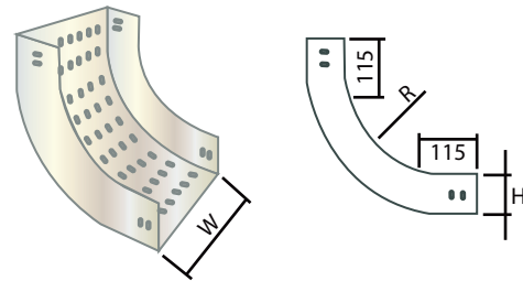
RADIUS
