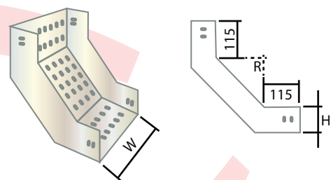
DIAGONAL
